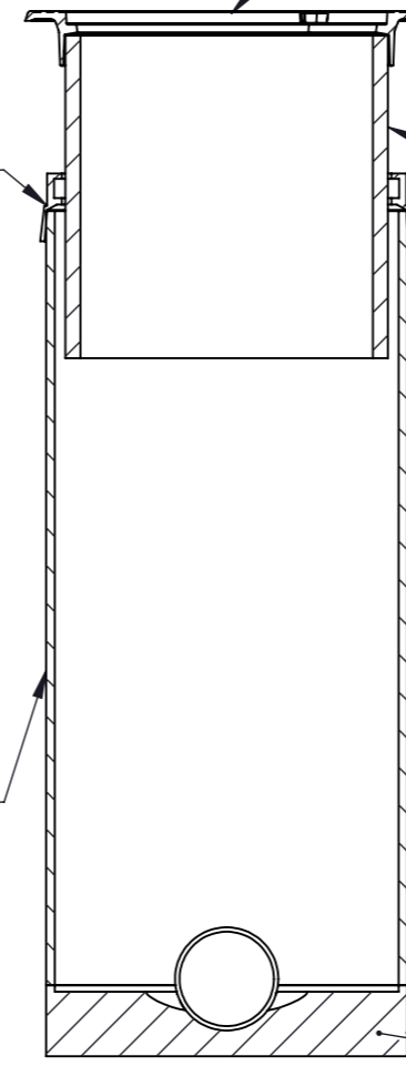
SECTION C-C SCALE 1 : 13
