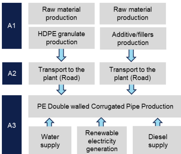
Figure 1 System boundaries of pipe manufacturing
